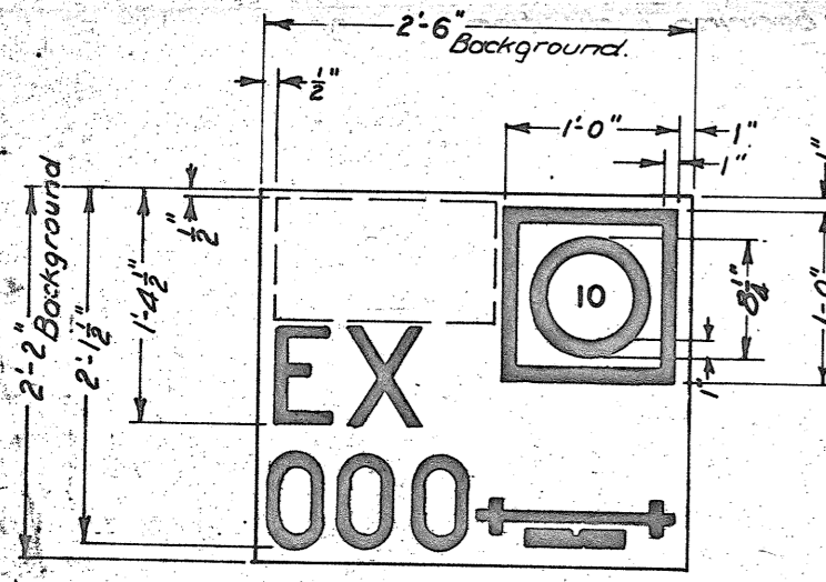
DETAIL OF LETTERING & MARKING PATCH
